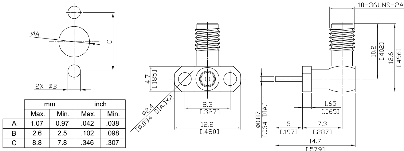
Mounting Dimensions
